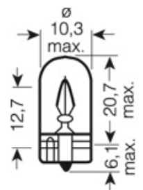
127 5511, 127 5322, 127 5528, W3W, W5W, WY5W
