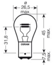
P21W, P21/4W, P21/5W, PY21W, PR21W, PR21/5W
