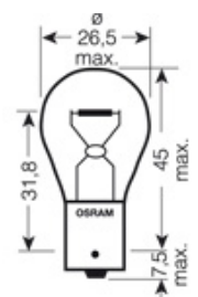
P21W, P21/4W, P21/5W, PY21W
